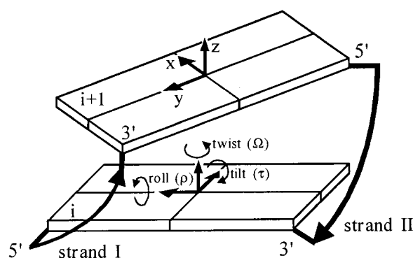
FIGURE 3 Orientational parameters of the basepair average plane in a dinucleotide step.
