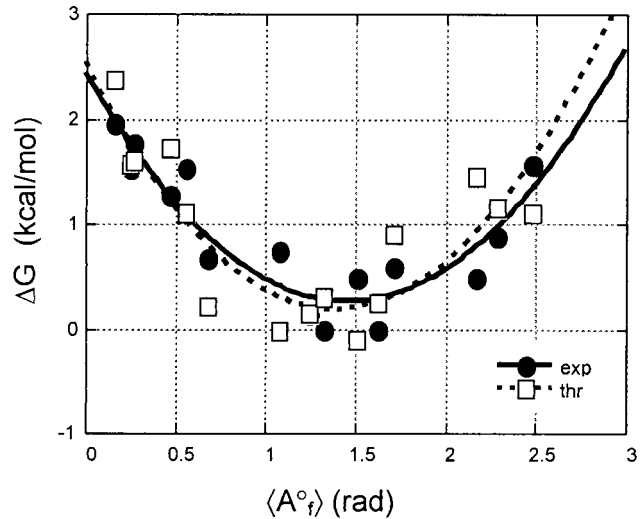
FIGURE 9 Experimental (●) and theoretical (□) nucleosome reconstitution free energy versus the effective curvature \langle A_f^\circ \rangle for a homogeneous pool of DNA fragments of the same length ( N = 162 bp), investigated by Shrader and Crothers (1989, 1990).
