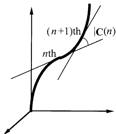
FIGURE 2 Representation of the DNA curvature as the angular deviation between the local helical axes of the turn centered on the n th and (n + 1) th basepairs.
